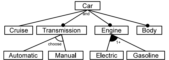
Figure 12: Feature diagram
