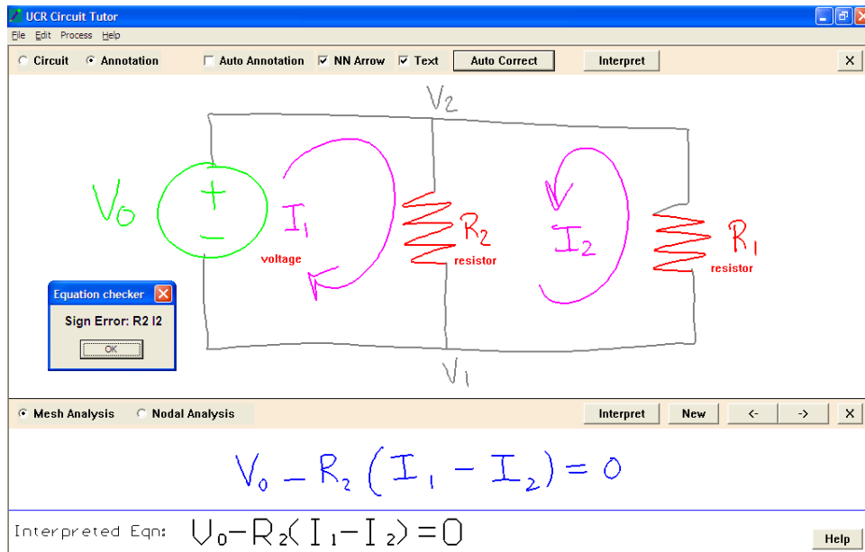
Figure 1: Kirchhoff's Pen used for mesh analysis. The system informs the student of the sign error on the " R_2I_2 " term.
