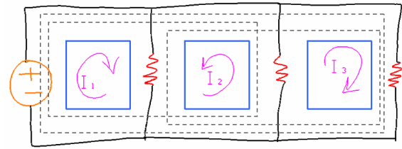
Figure 2: Circuit with six meshes indicated by approximately inscribed rectangles (3 dashed, 3 solid). The three solid rectangles indicate "windows," meshes that are preferred for analysis.
