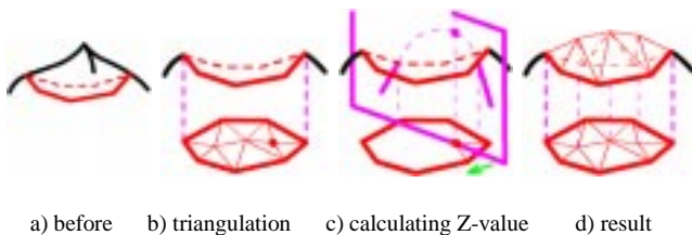
Figure 21: Smoothing algorithm.
