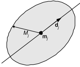
Fig. 1. Example of the geometric representation of an EAM category j when the feature space is two-dimensional. \mathbf{m}_j is the center of the ellipsoid, \mathbf{d}_j is the orientation vector, coinciding with the direction of the major axis of the ellipsoid, and M_j is the Mahalanobis radius of the category.
