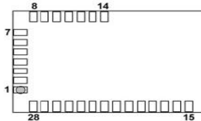
Figure 21 Laird BT800 pin layout
