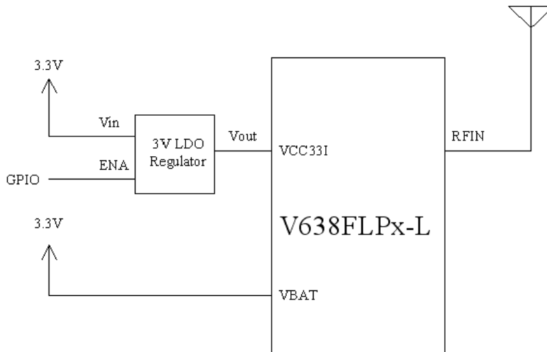
Figure 18 Venus638FLPx-L sleep mode schematic
