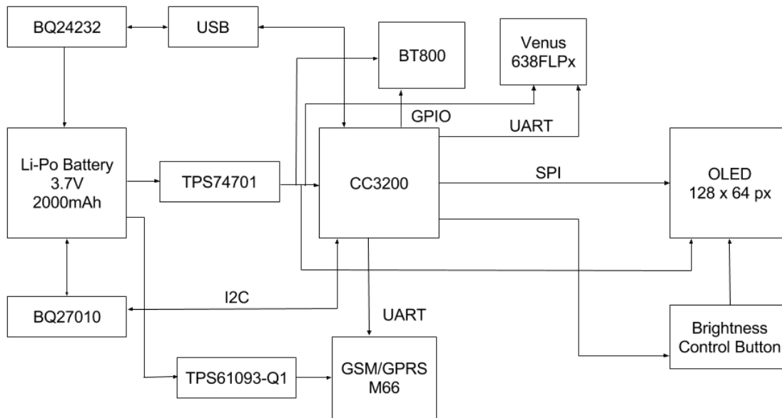
Figure 16 Final Watch Block Diagram
