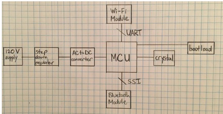
Figure 22 Final Block Diagram
