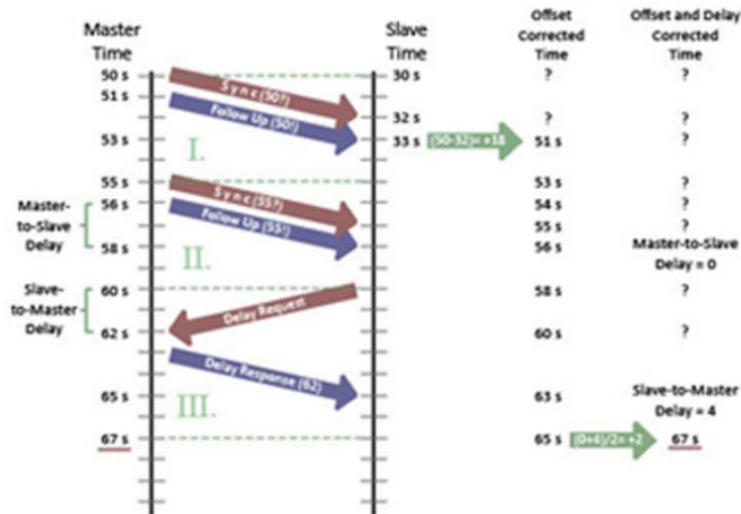
Figure 20 Bidirectional Multicast Communication (Courtesy of Real Time Automation, Inc.)
