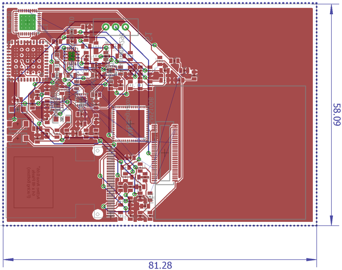
Figure 28 Example of PCB watch hardware
