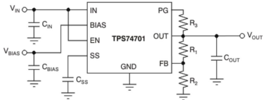
Figure 13 TPS74701 pin connections (Courtesy of Texas Instruments)
