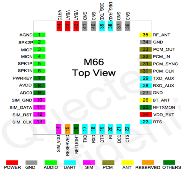
Figure 7 Quectel M66 PIN Layout (Courtesy of Quectel)
