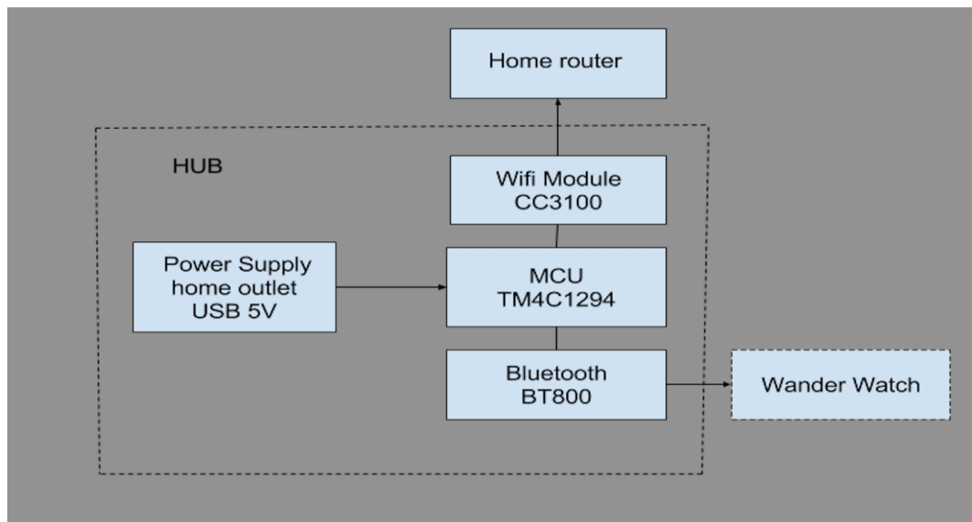
Figure 19 Hub Block Diagram
