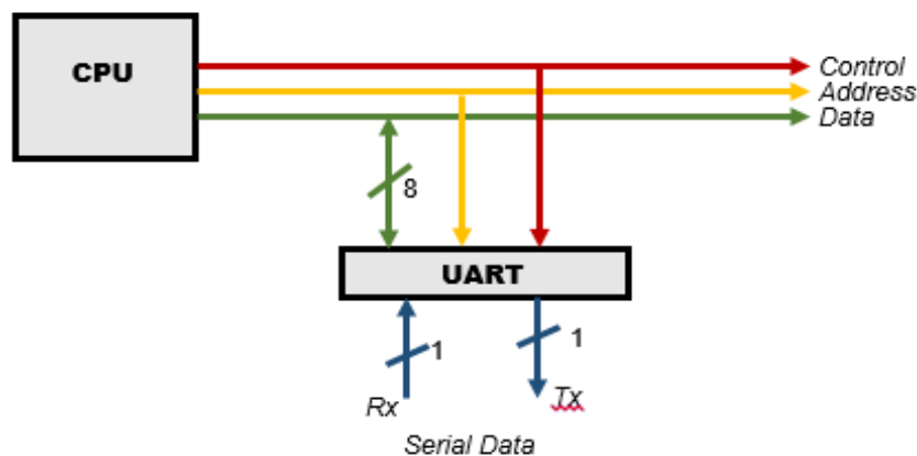
Figure 5 UART serial and parallel control lines
