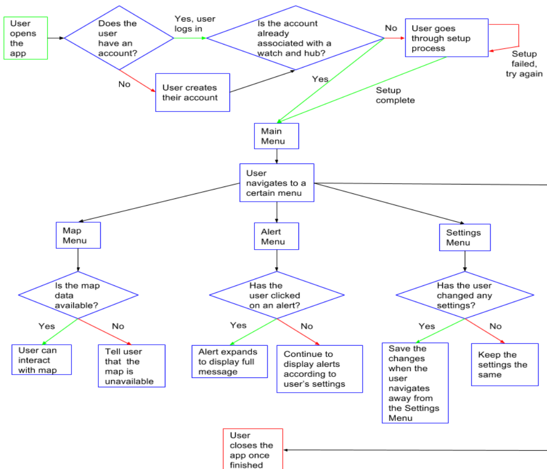
Figure 24 Control flow diagram for the Wander Watch application
