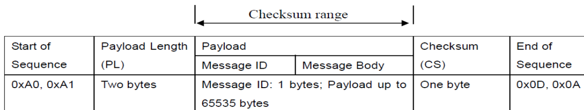
Figure 30 Venus638FLPx-L binary message format
