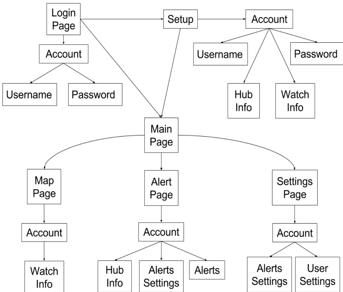
Figure 26 Data structure diagram for the Wander Watch application
