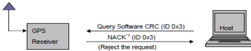
Figure 32 Host Computer to GPS receiver NACK communication
