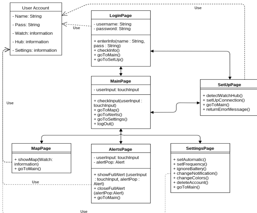
Figure 25 UML class diagram for the Wander Watch application
