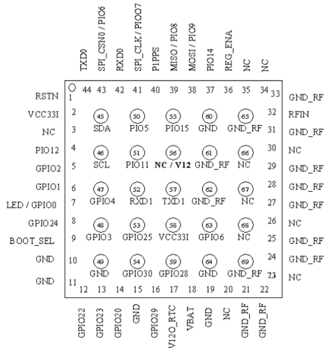
Figure 17 Venus638FLPx-L pin layout
