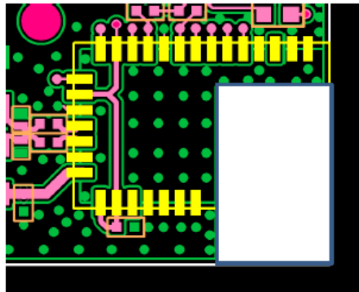
Figure 29 The Laird BT800 “Antenna Keep-out Area” can be seen here in white.
