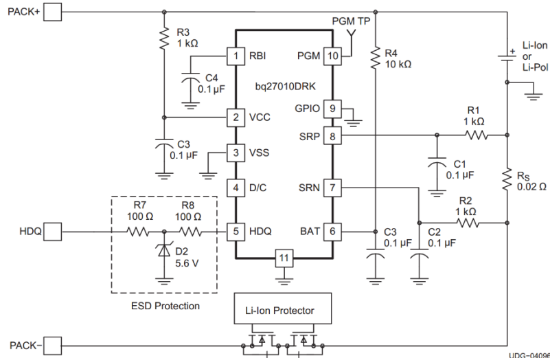
Figure 15 BQ27010 fuel gauge application (Courtesy of Texas Instruments)
