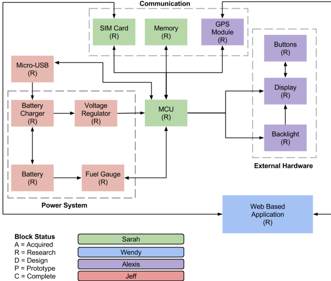
Figure 10 Block Diagram
