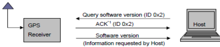
Figure 31 Host Computer to GPS receiver ACK communication
