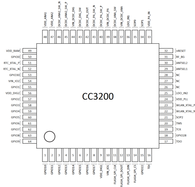
Figure 11 CC3200 pin layout (Courtesy of Texas Instruments)
