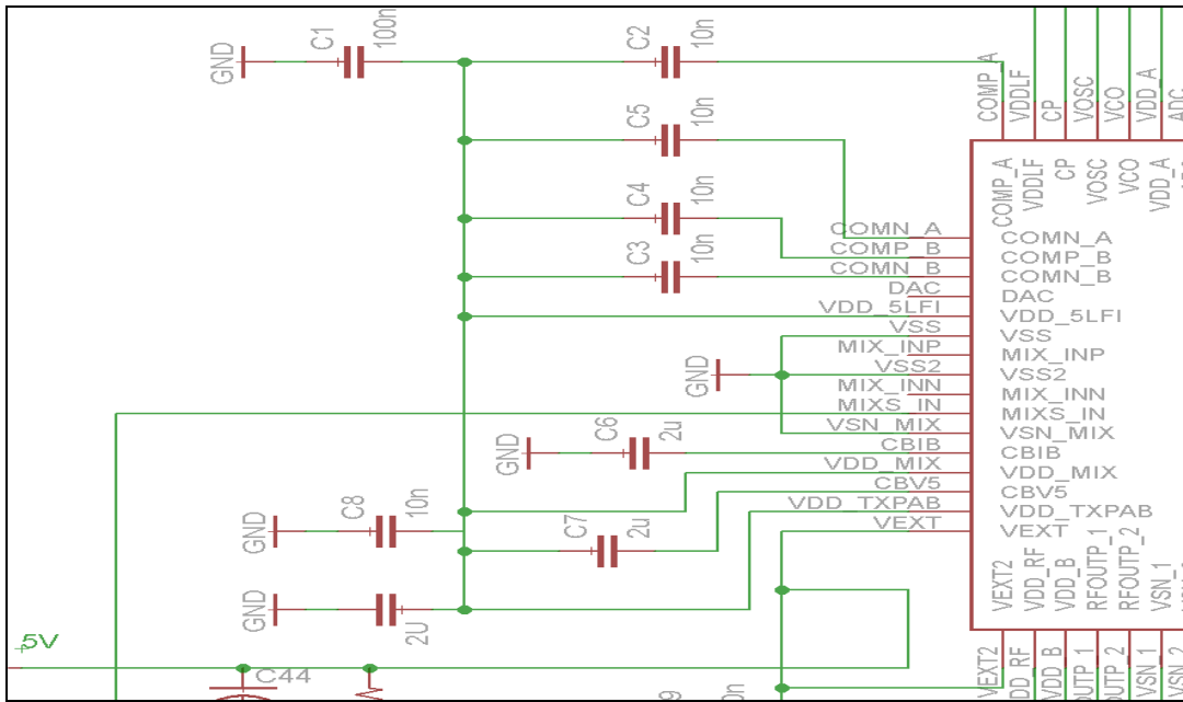
Figure 25 – Reader Schematic for pins 1-17 and 64
