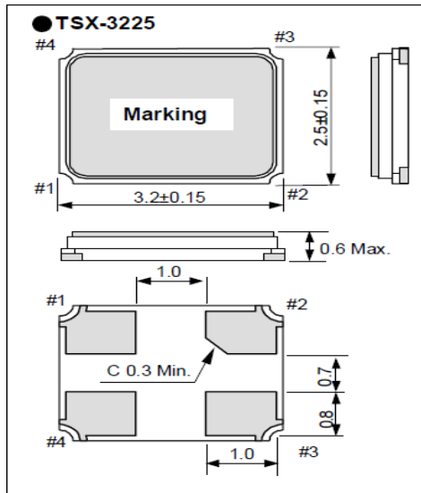
Figure 30 – TSX-3225 Dimensions
