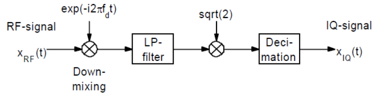
Figure 24 – IQ Demodulator
