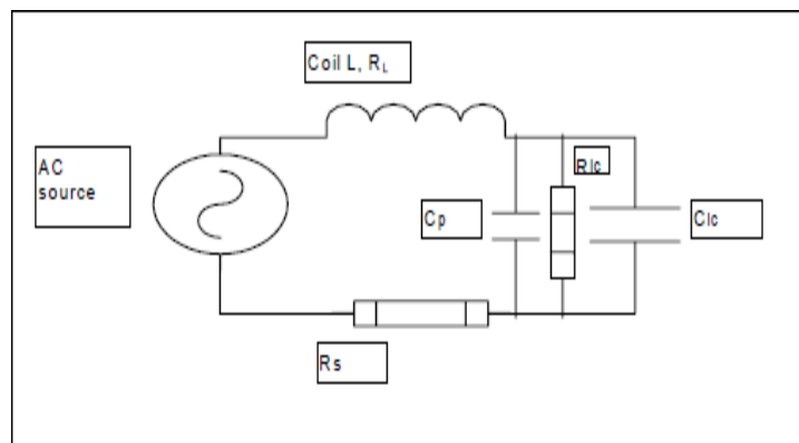
Figure 6 - Tag resonator
