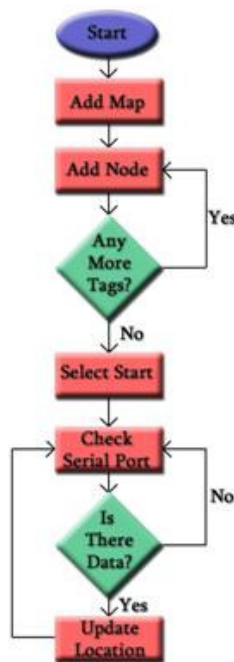
Figure 46 - Flow chart for the GUI
