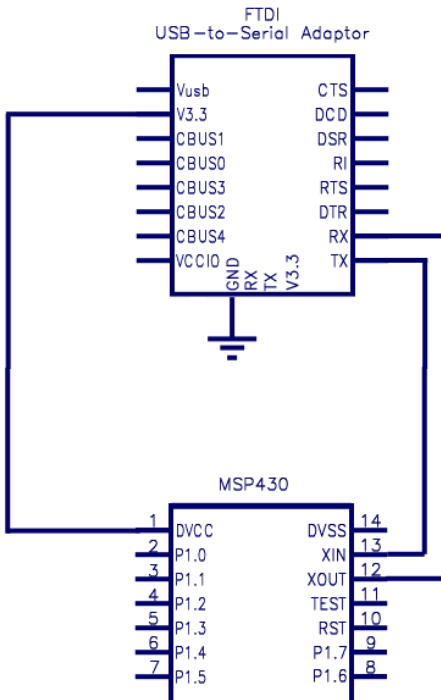
Figure 48 - MSP430/Bob layout
