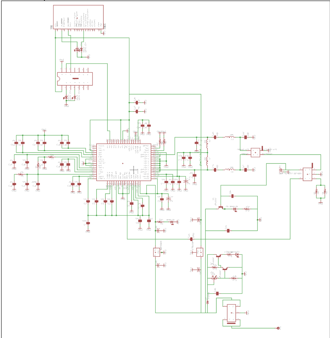
Figure 45 – Complete Reader Schematic
