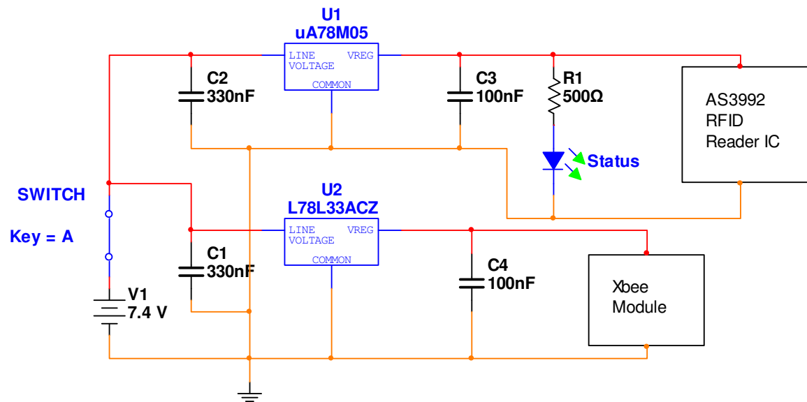
Figure 16 - Power circuit for the reader unit
