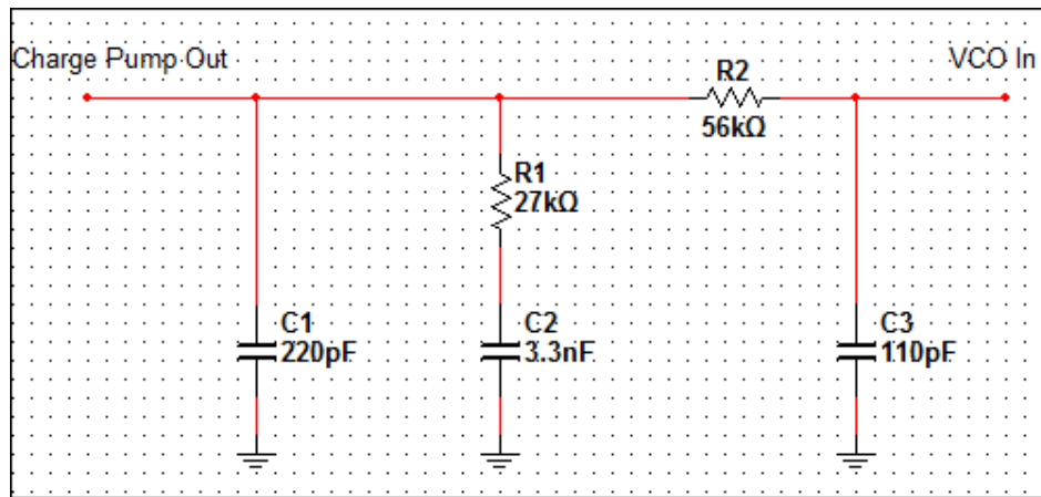
Figure 22 – Loop Filter Circuit
