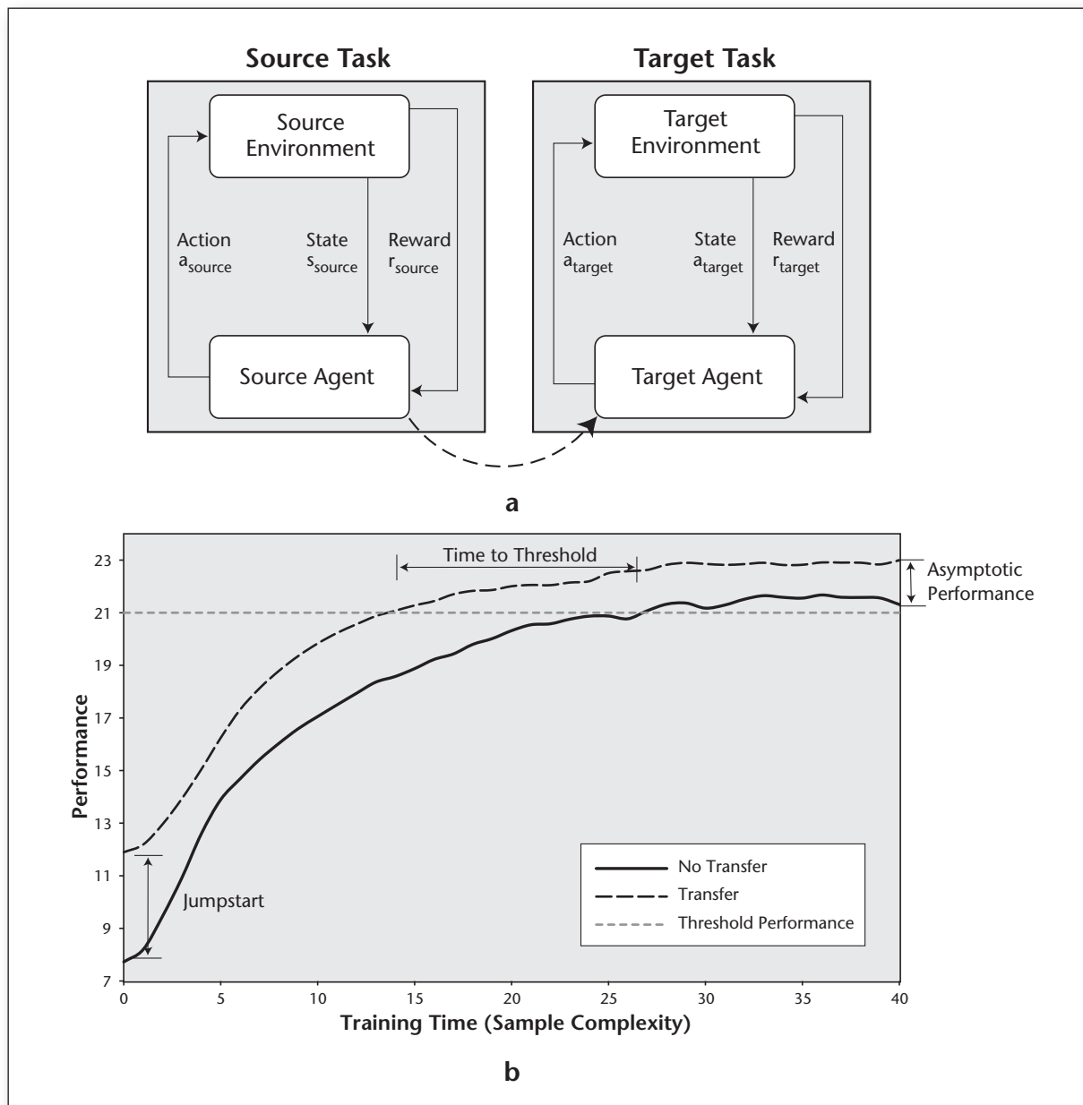
Figure 4. Transfer in RL.
