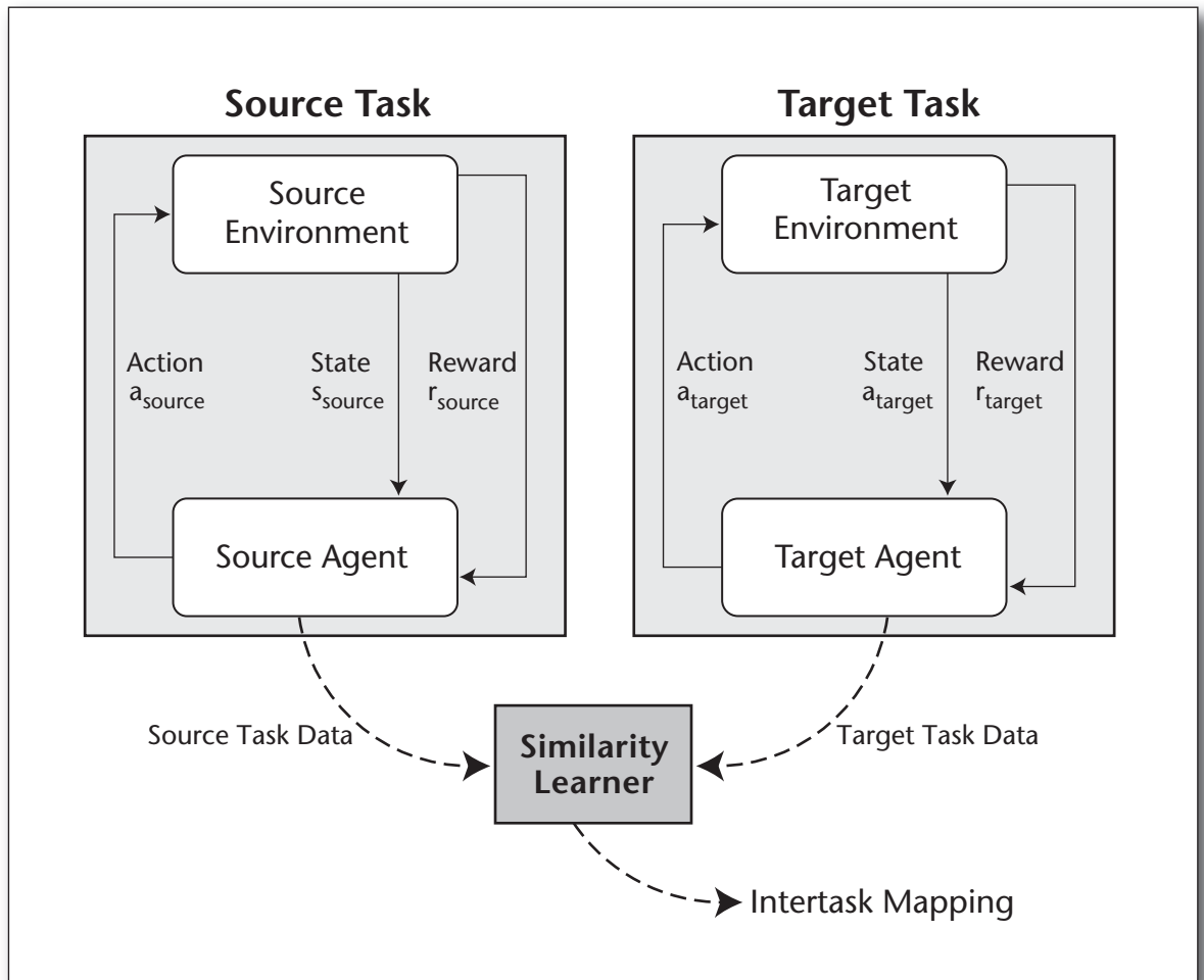
Figure 11. One Class of Methods to Learn Intertask Mappings.
