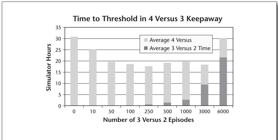
Figure 9. One Set of Results in a Simulated Soccer Goal Scoring Task.
