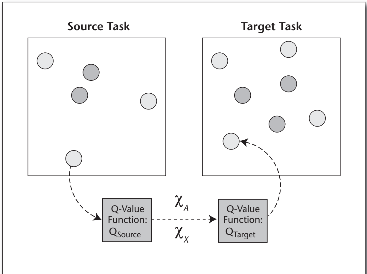
Figure 7. In Value Function Transfer, Learned Q-Values from the Source Task Are Transformed through Intertask Mappings.
