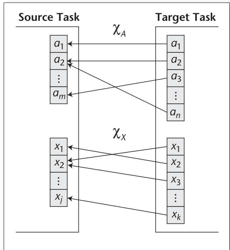
Figure 6. \chi_A and \chi_X Are Independent Mappings that Describe Similarities between Two MDPs.
