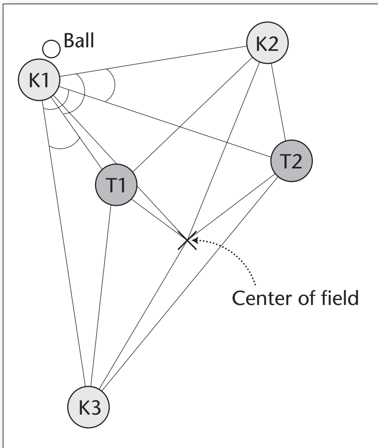
Figure 2. The Distances and Angles Used to Construct the 13 State Variables Used in 3 versus 2 Keepaway.
