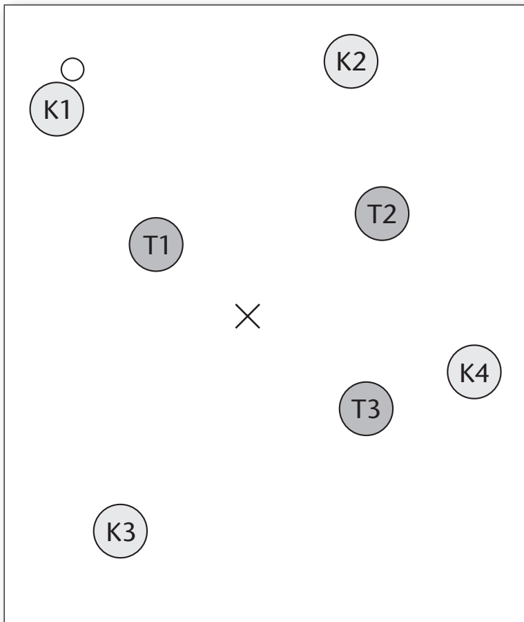
Figure 3. 4 Versus 3 Keepaway
