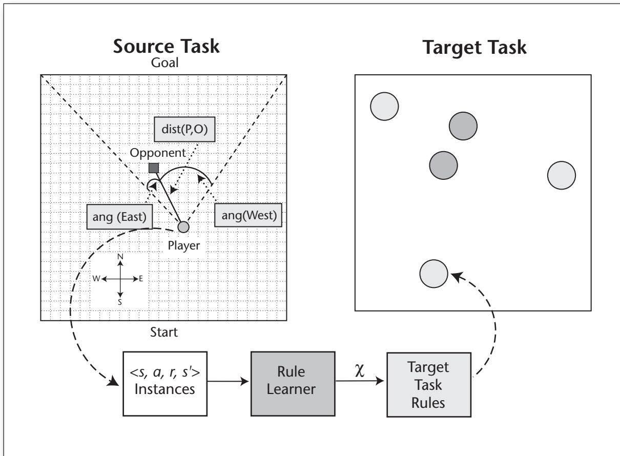
Figure 10. Interdomain Transfer Can Result in Significant Improvements to the Total Learning Time Required.
