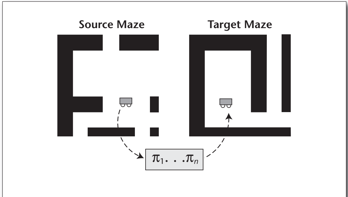
Figure 5. Many Methods Directly Use a Learned Source-Task Policy to Initialize an Agent's Policy in the Target Task, or to Bias Learning in the Target Task.
