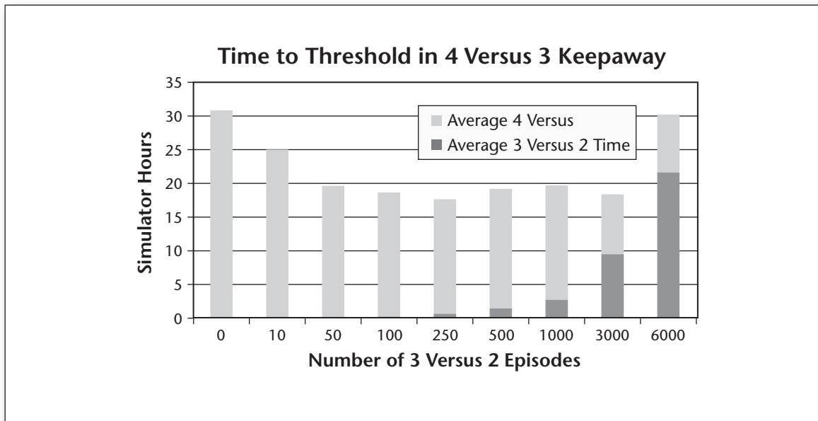
Figure 8. Some Results from Value Function Transfer Work.
