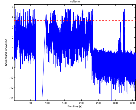
Fig. 3. The log of the normalized innovation of the EKF for run 1. The dashed line shows \log(4) which should be the average value if the filter is consistent. The drop between 65s and 95s occurs because the tracker loses track and does not provide any observations.
