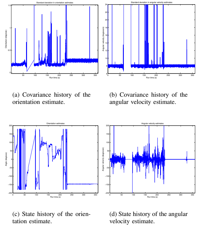
Fig. 4. Covariance histories and state estimates for run 1 using the KF.
