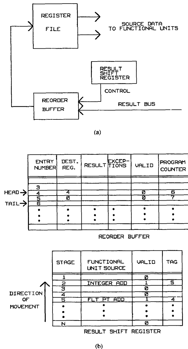
Figure 3. (a) Reorder Buffer Organization. (b) Reorder Buffer and associated Result Shift Register.
