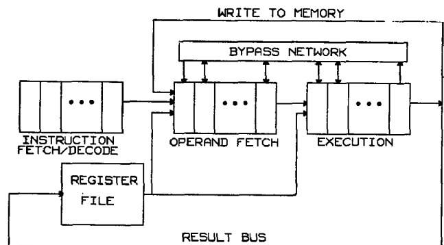
Figure 7. Example of a linear pipeline implementation.
