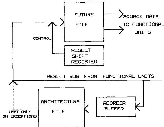
Figure 6. Future File Organization.
