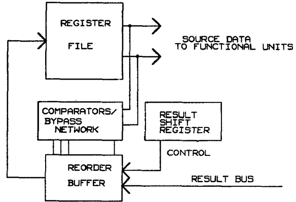
Figure 4. Reorder Buffer Method with Bypasses.
