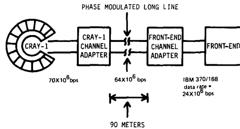
Fig. 8. Front-end system interface.
