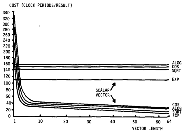
Fig. 7. Scalar/vector timing.
