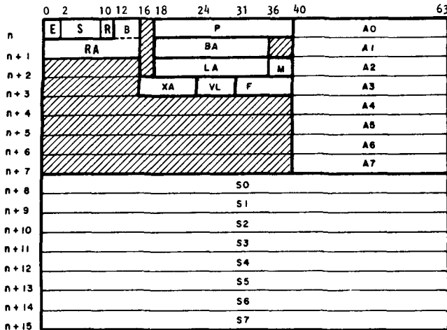
Fig. 6. Exchange package.
