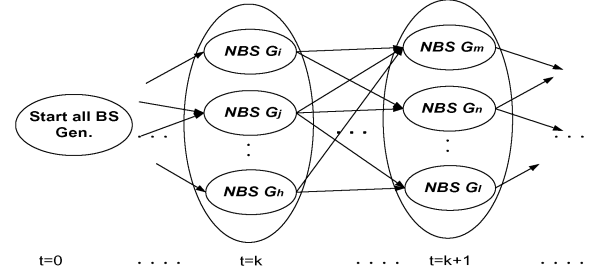
Fig. 6. Dynamic programming.
